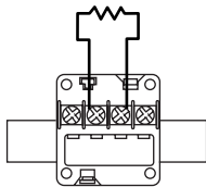
KwikLink IDC with open-style terminator
